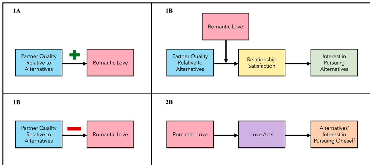
Fig. 2. Predictions of Frank (1988)'s classic commitment device hypothesis and the signaling-to-alternatives hypothesis.
